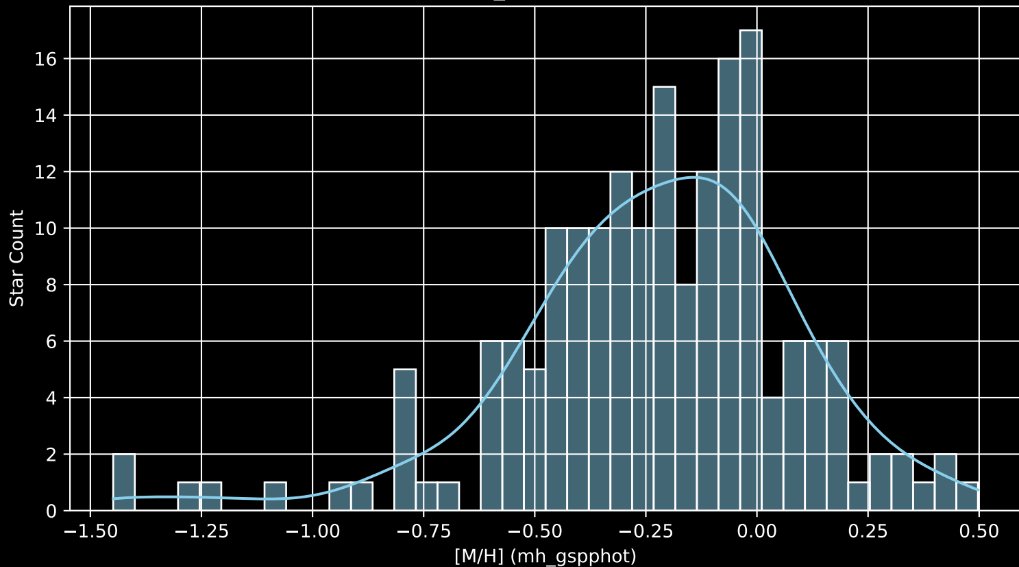
APOGEE DR17 Field: [193+25_MGA [M/H] (mh_gspphot) (n= 182)
