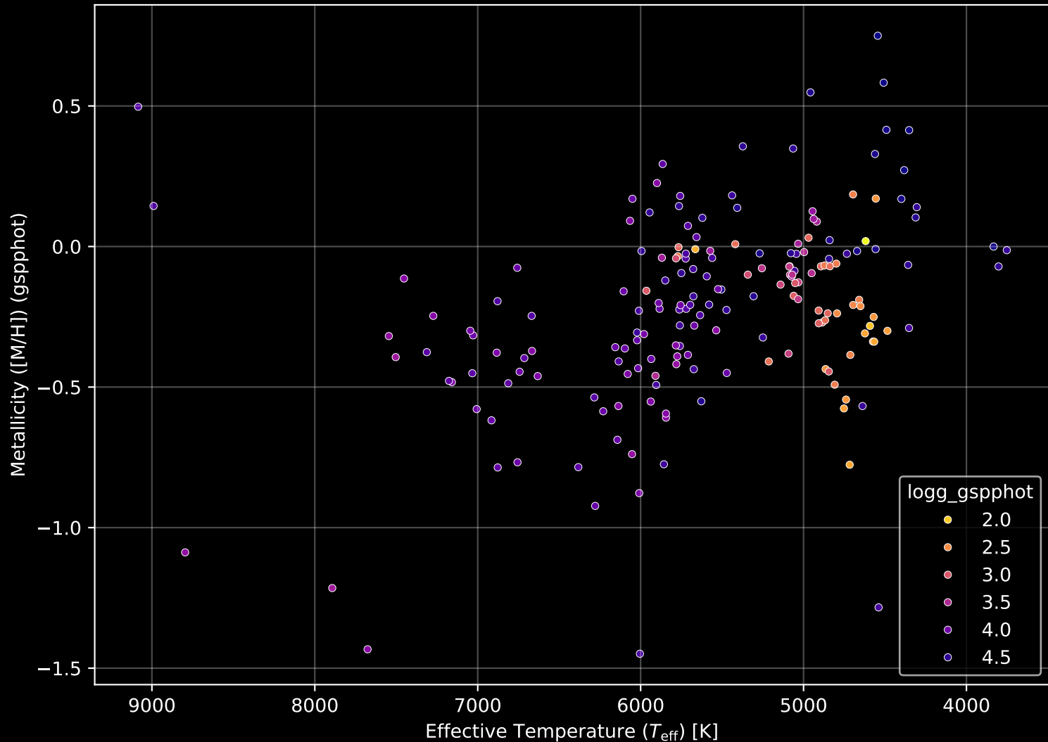
APOGEE DR17 Field: [193+25_MGA] Stellar Population Parameters (n= 185)
