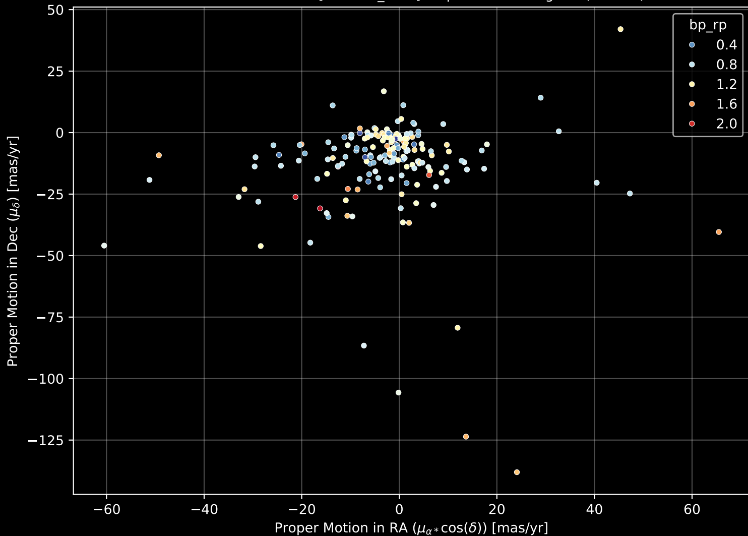
APOGEE DR17 Field: [193+25_MGA] Proper Motion Diagram (n= 185)
