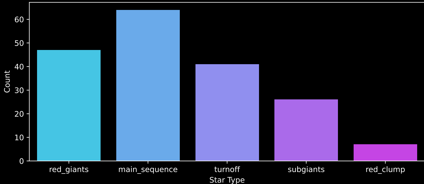
APOGEE DR17 Field: [193+25_MGA] Count plot of Star Type
