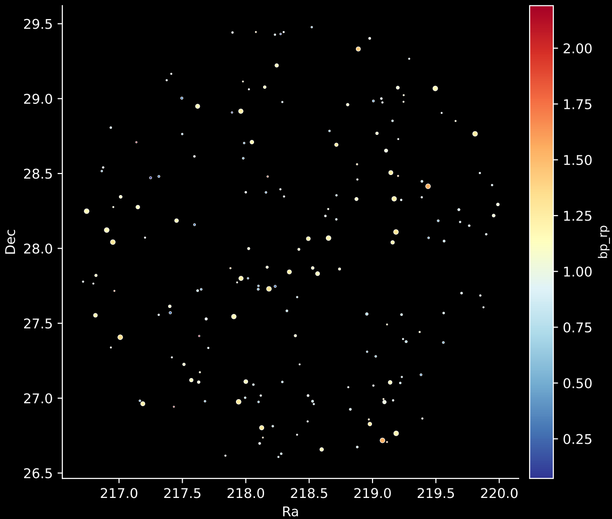
APOGEE DR17 Field: [193+25_MGA] Stars: 185
