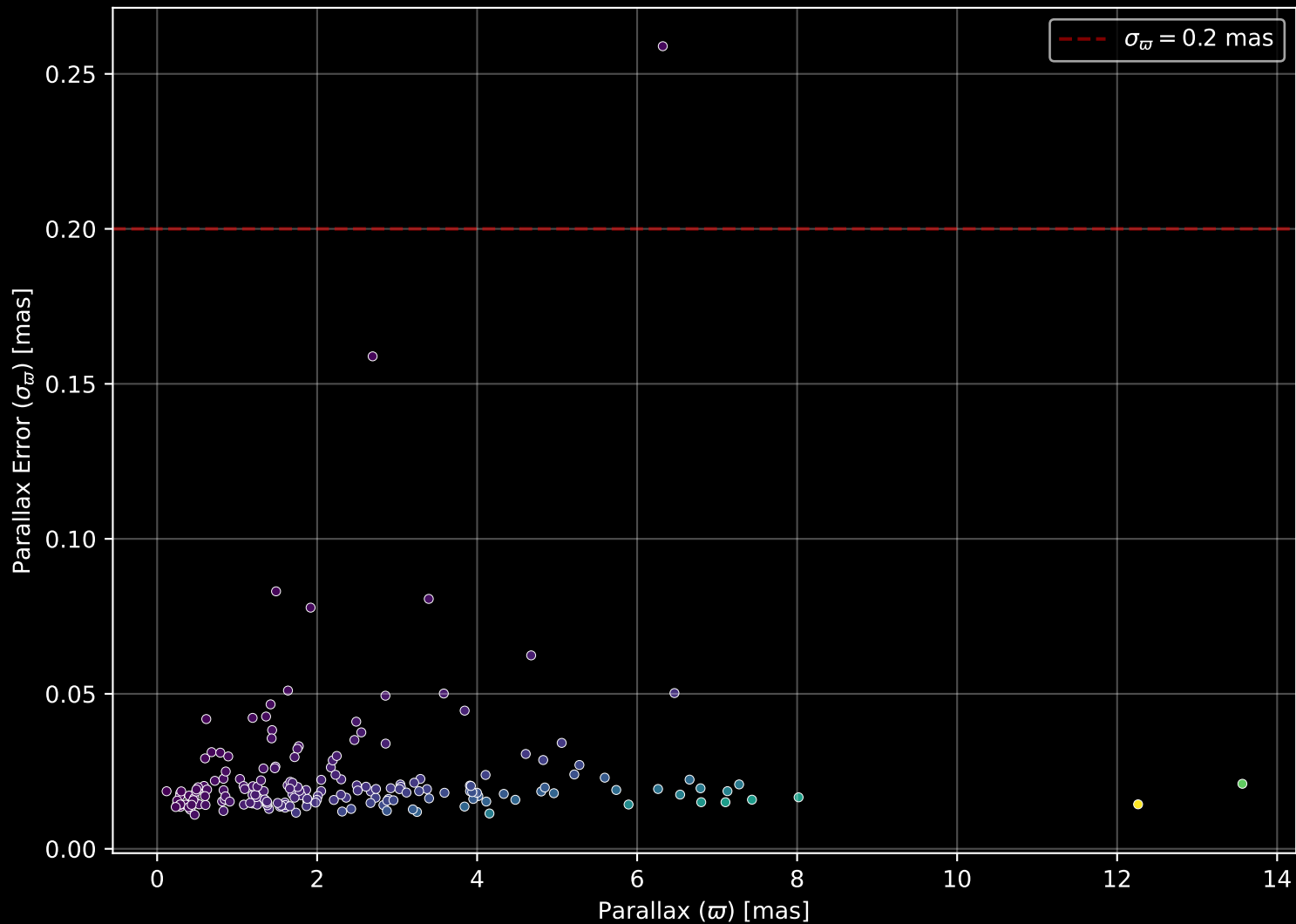
APOGEE DR17 Field: [193+25_MGA] Parallax Quality (n= 185)
