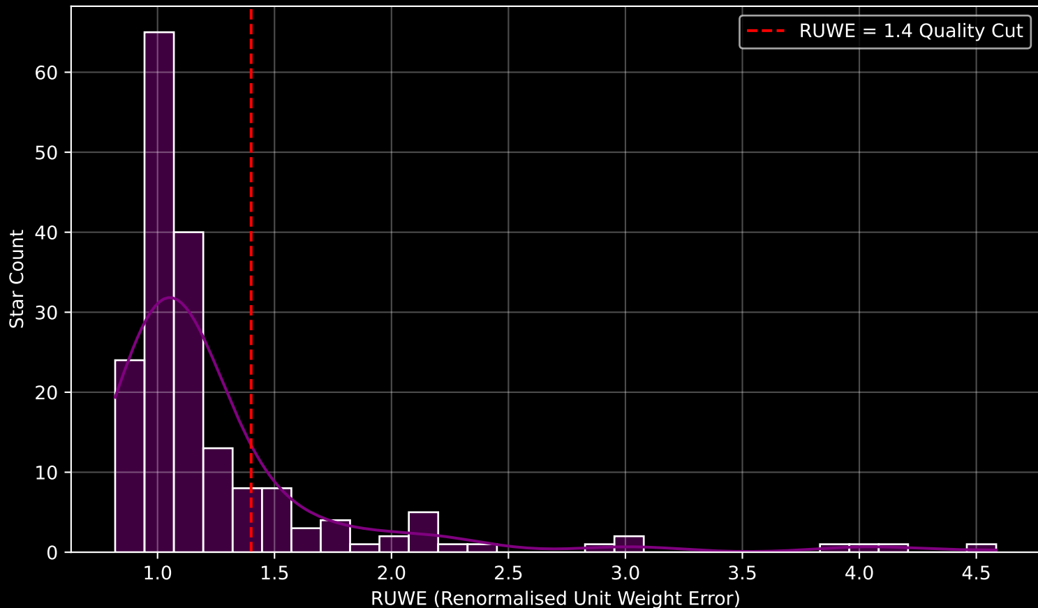
GAPOGEE DR17 Field [193+25_MGA] RUWE Distribution (n= 182)
